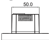
⑥ TOP VIEW
